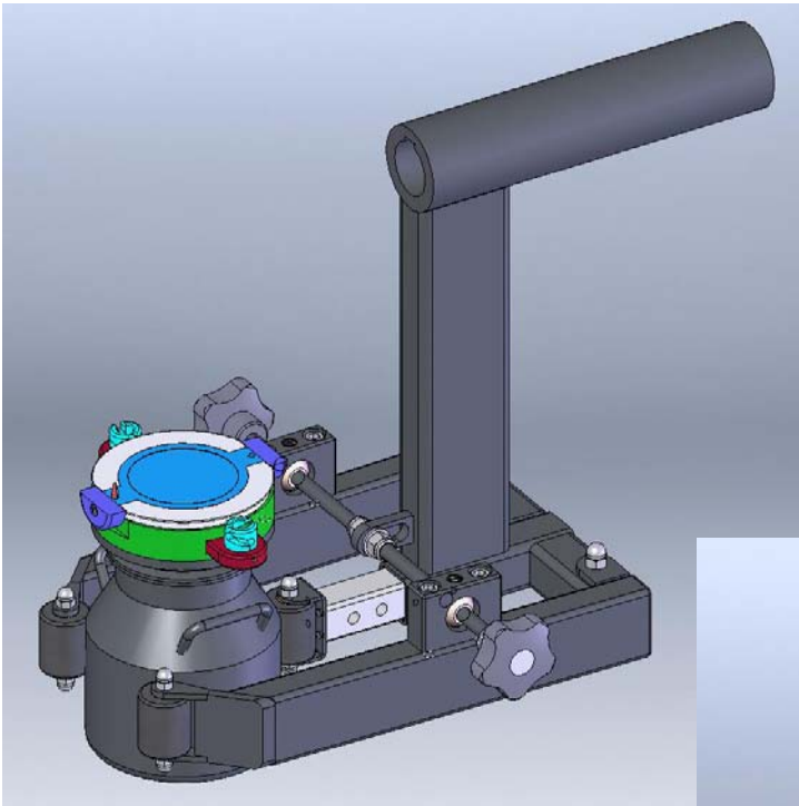
5 lt vessel with passive split valve
