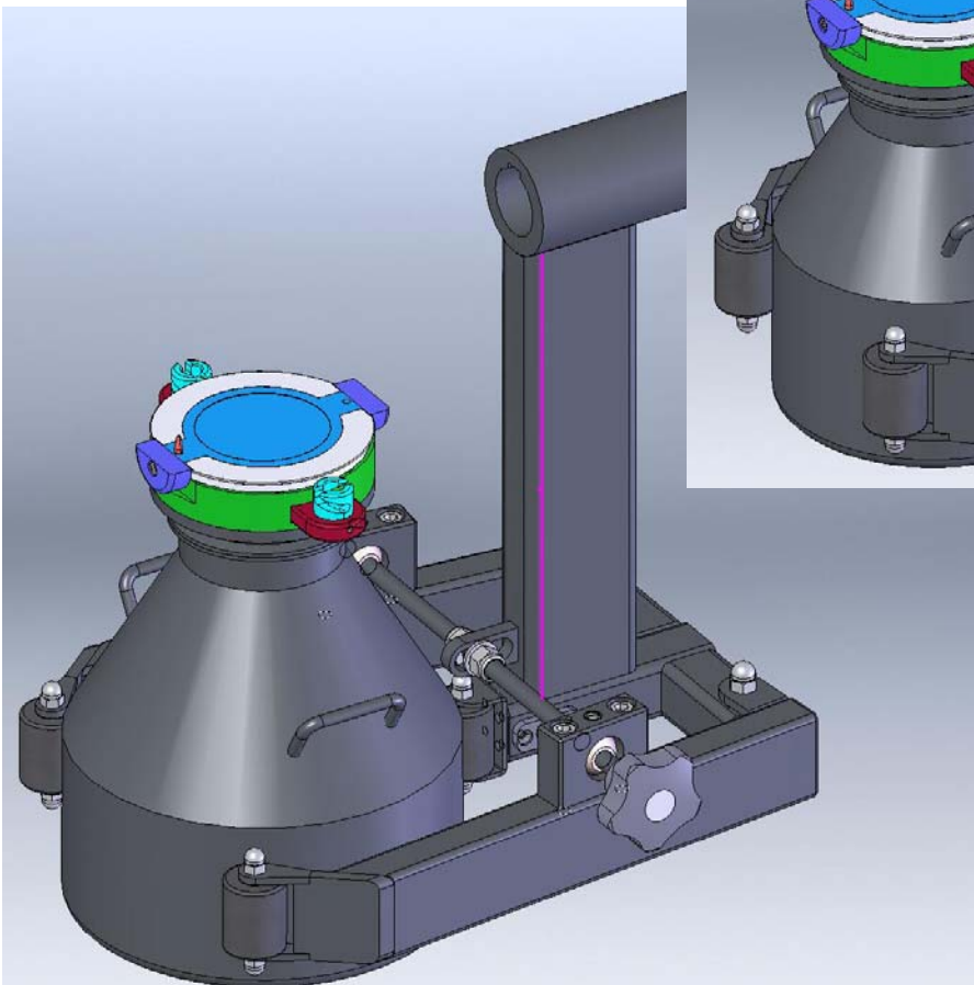
10 lt vessel with passive split valve
