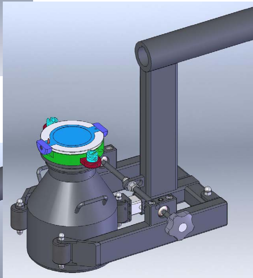
5 lt vessel with passive split valve
