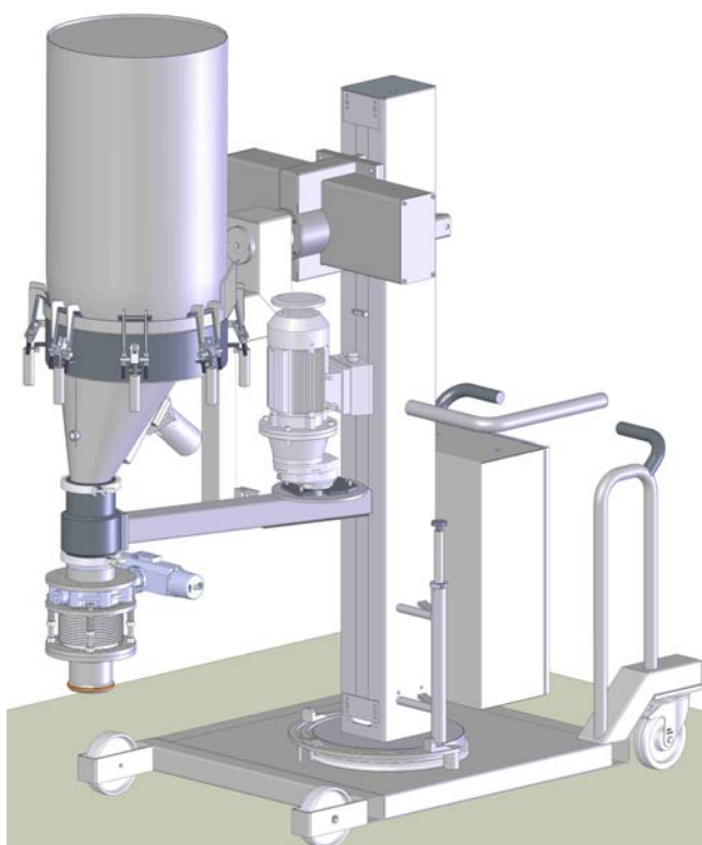
Unloading drum
