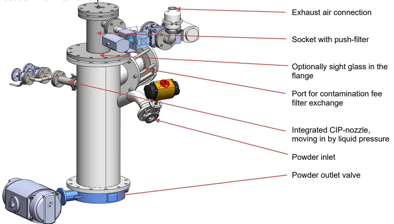
Execution with filter on top
