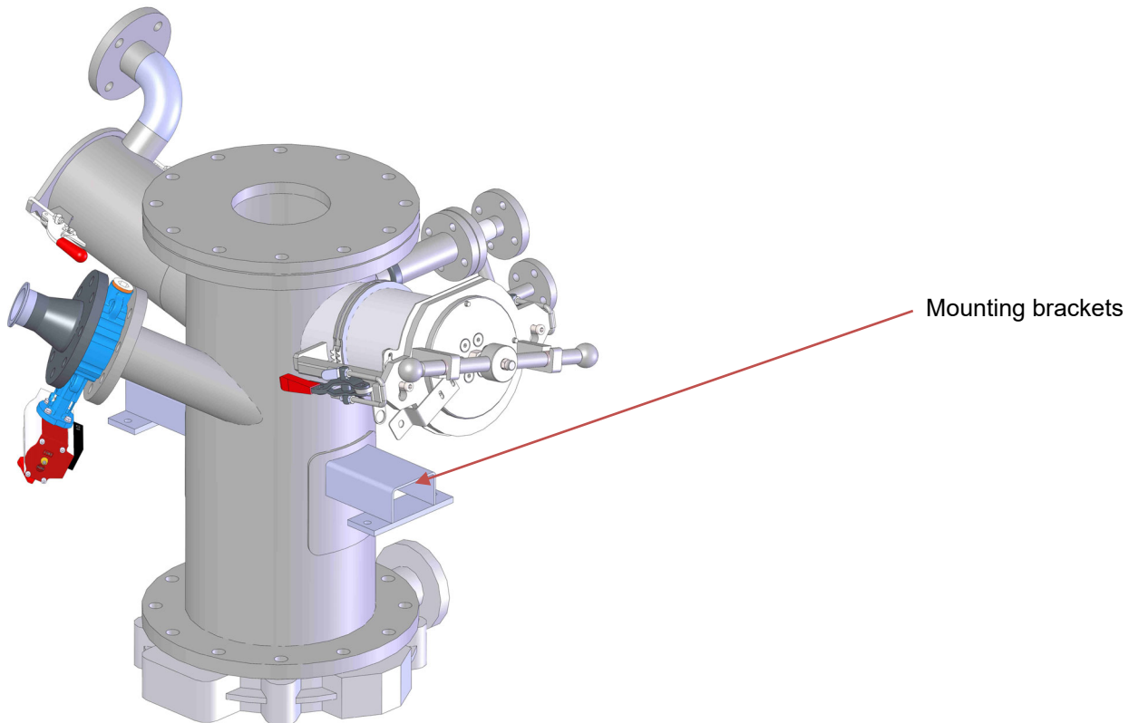
Execution with filter in the cylindrical part
